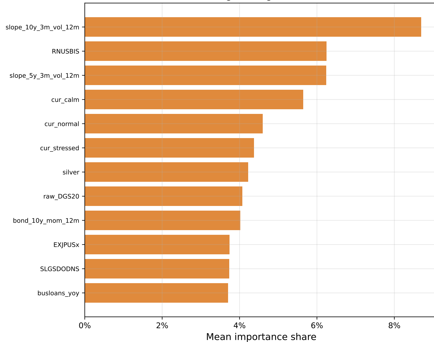
Logistic regression
