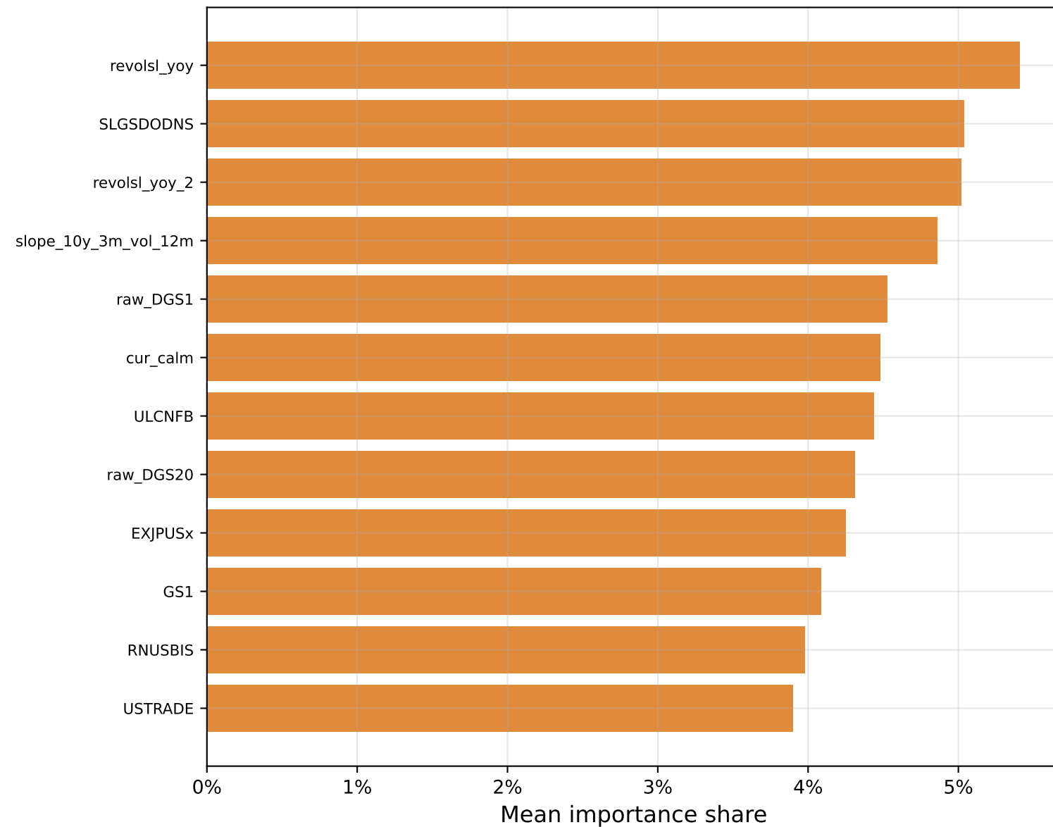
Random forest
